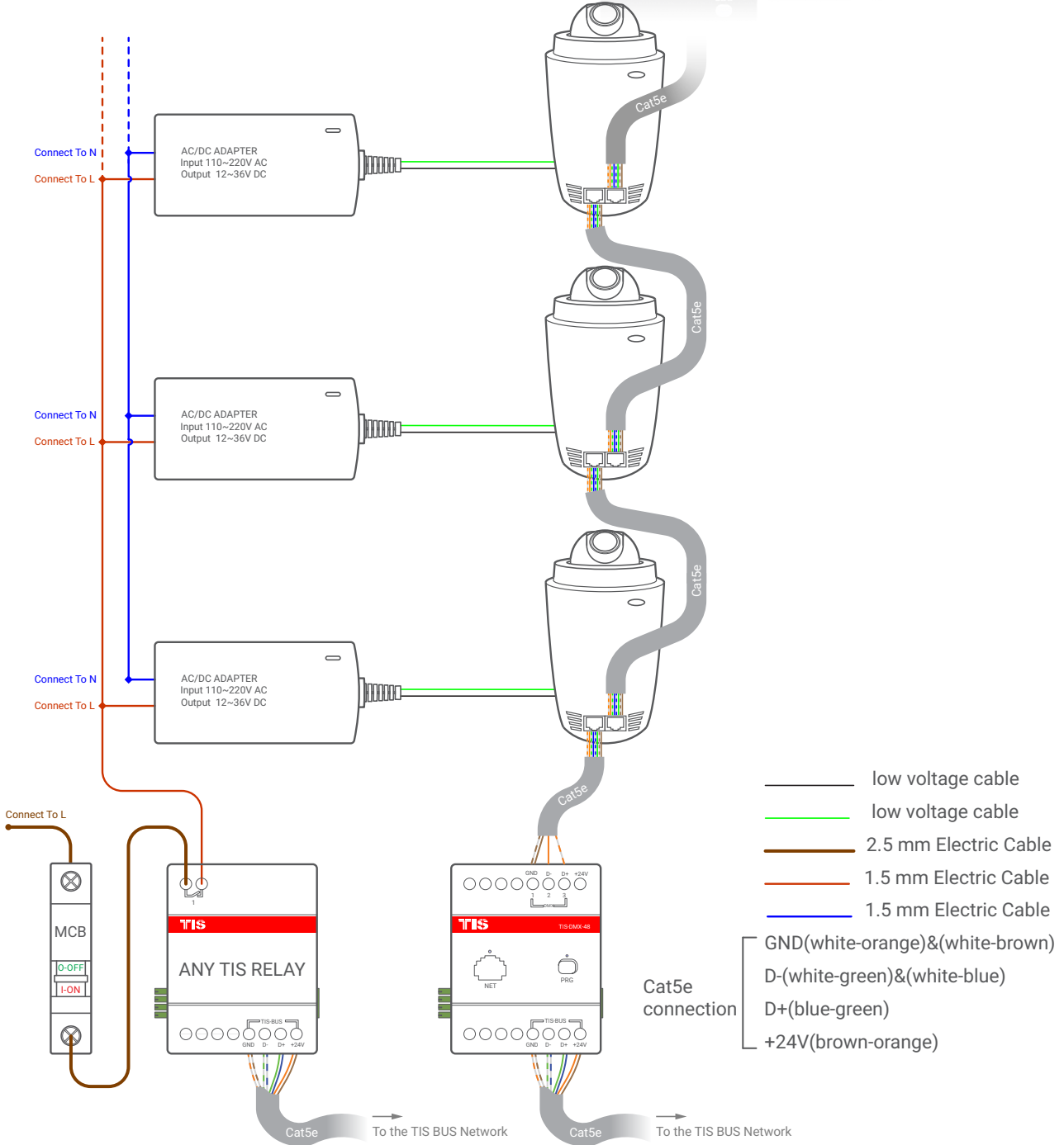
▲ Figure 1: DMX Lights Connection Diagram
