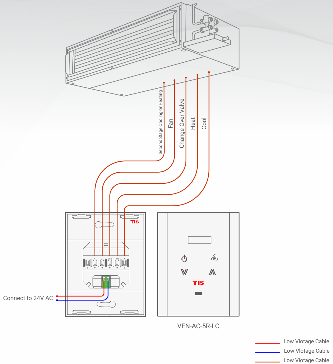
▲ Figure 1: VEN-AC-5R-LC & FCU Connection Diagram
