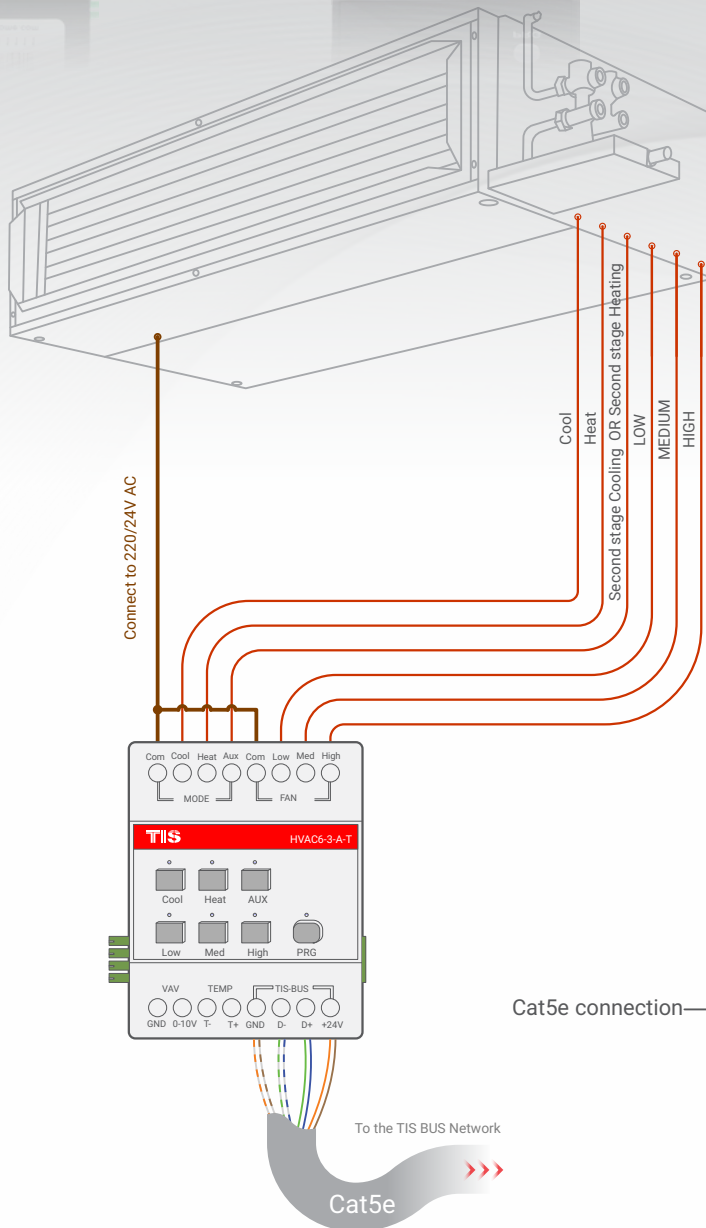
▲ Figure 1: FCU Connection Diagram
