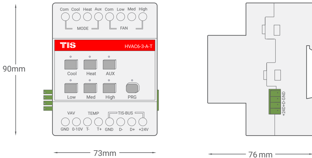
▲ Figure 4: Module's Dimensions
