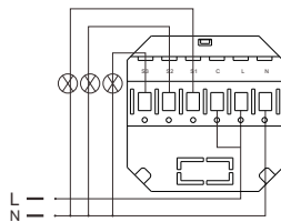
ADS 3 Relay Controller ADS-3R-3Z
