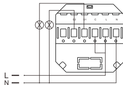
ADS 2 Relay Controller ADS-2R-2Z
