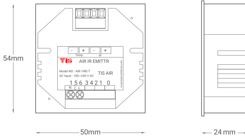
▲ Figure 2: Module Dimensions
